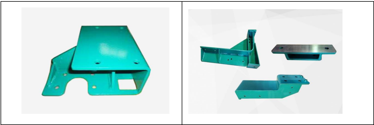
5. Deep Drawn Parts- Deep Draw Components for Pneumatic Actuators- Made out of Mild steel Plates, Used in Control Automation.
